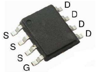
SOP-8
